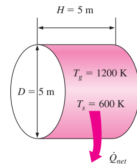
FIGURE 12–40 Schematic for Example 12–14.
