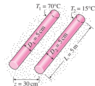
FIGURE 3-50 Schematic for Example 3-14.
