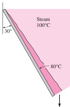
FIGURE 10-31 Schematic for Example 10-5.
