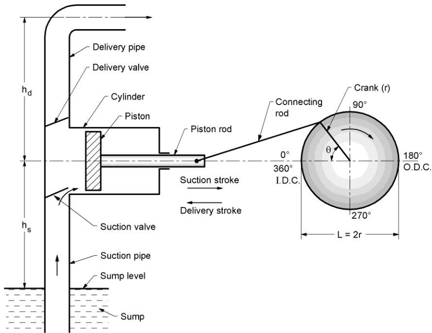
Fig. 10.1 Main parts of reciprocating pump
