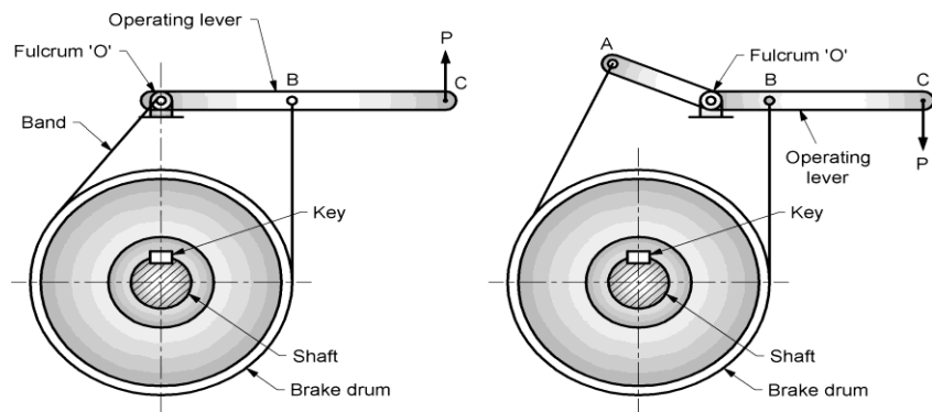
Fig.7.13 Band Brake
