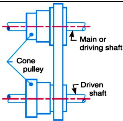
Fig. 8.12 Stepped/Cone pulleydrive
