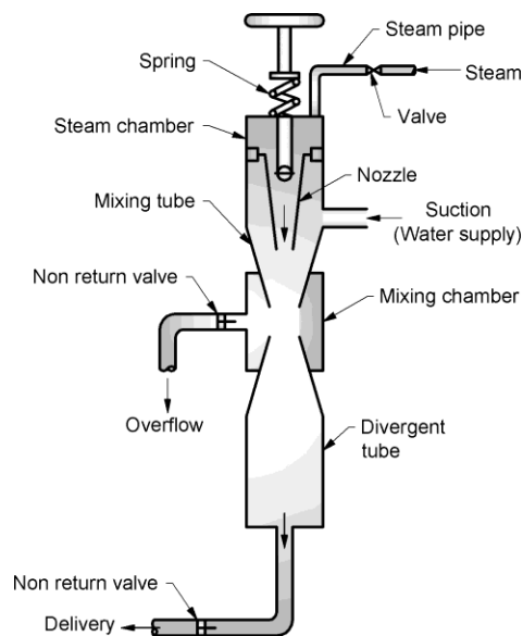
Fig. 2.18 Steam injector
