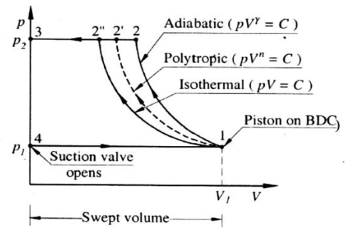
Fig. 5.4 P-V Diagram Neglecting Clearance Volume
