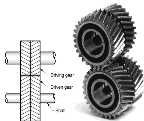
Fig.8.22 Doublehelical /Herringbone gear
