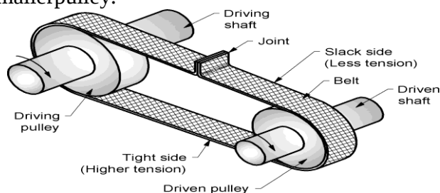
Fig 8.6 Belt Drive
