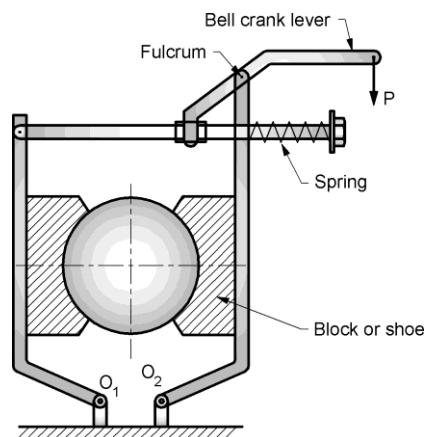
Fig. 7.12 Double block or shoe brake
