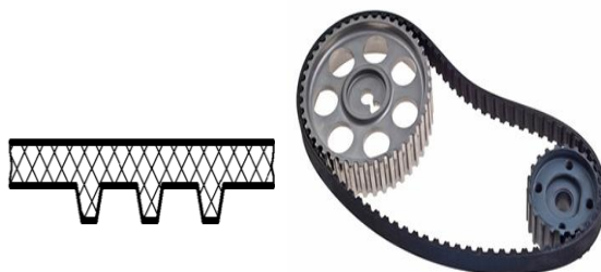
Fig.17 Timing belt
