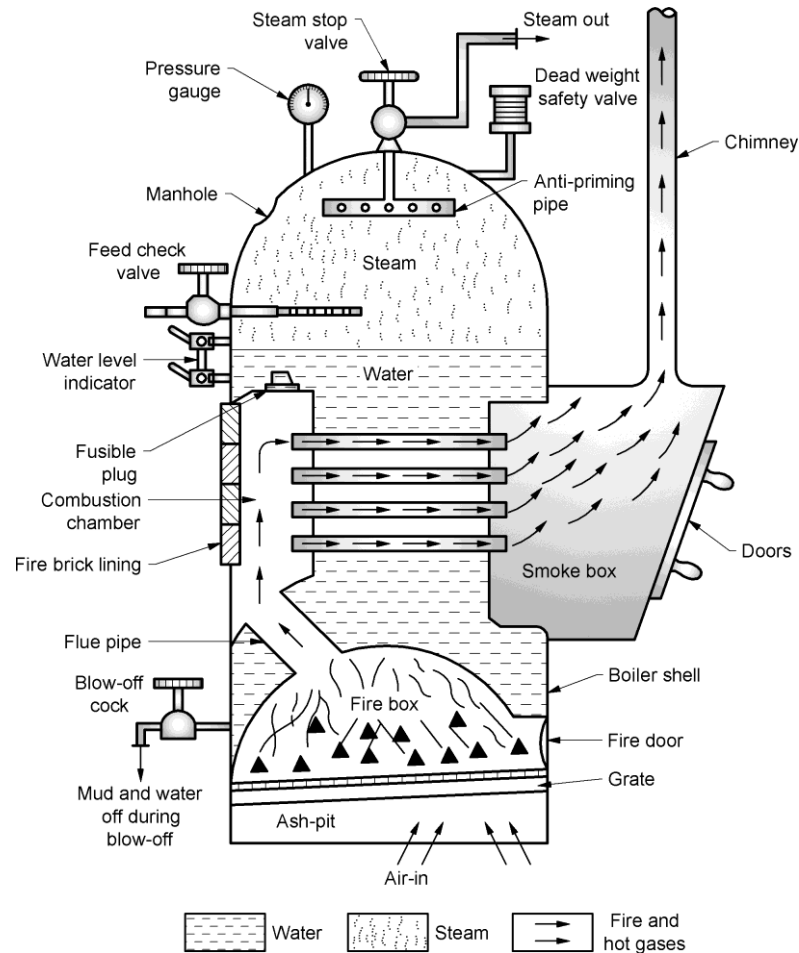
Fig. 1.3 Cochran Boiler
