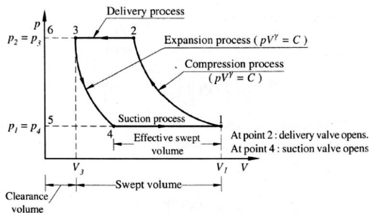
Fig. 5.5 P-V Diagram considering clearance volume
