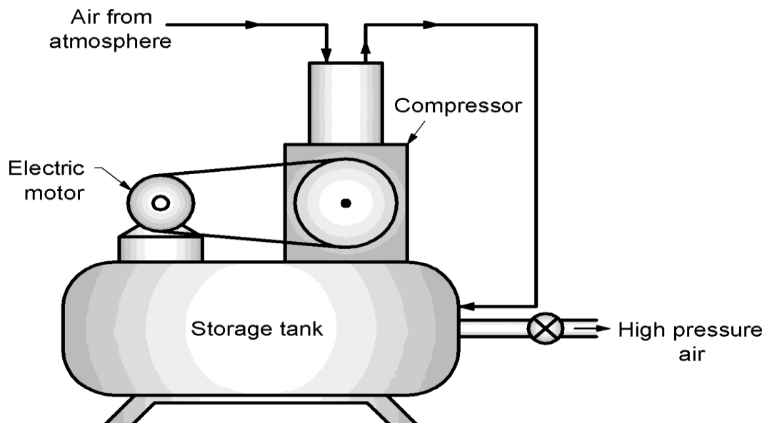
FIG. 5.1 AIR COMPRESSOR
