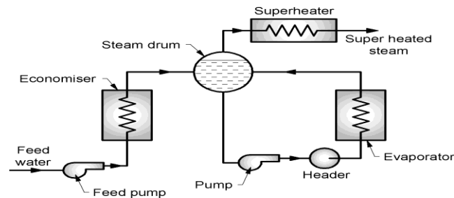
Fig. 1.2 Forced circulation boiler
