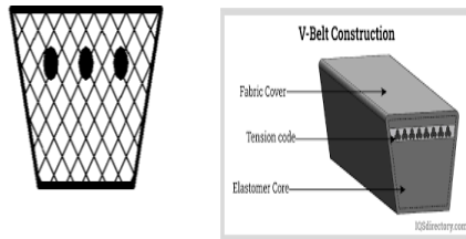
Fig.15 V belt
