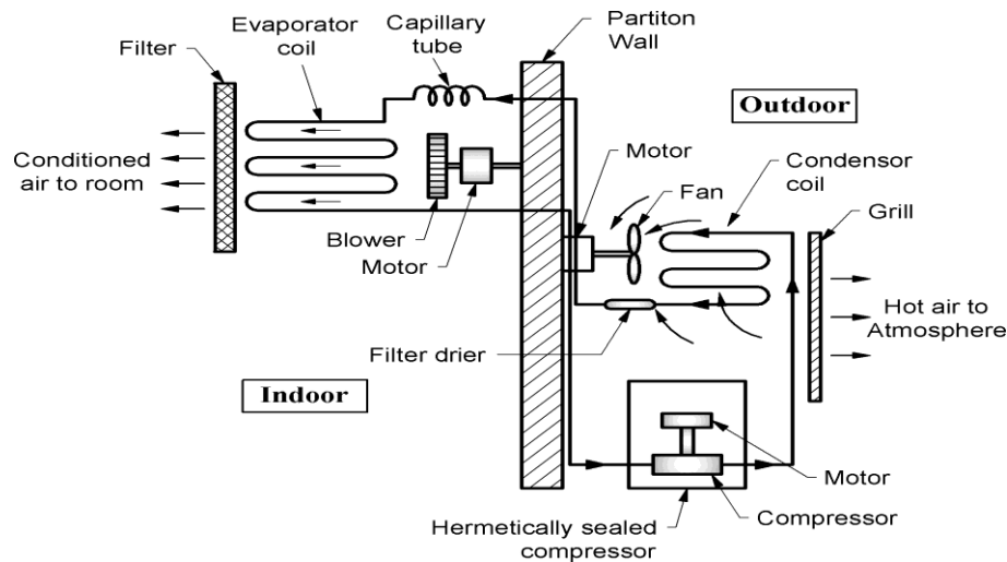
Fig.6.4:Split air conditioner
