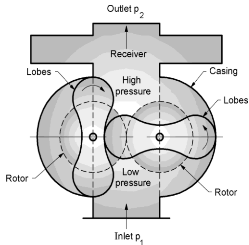
Fig.5.8, Roots Blower
