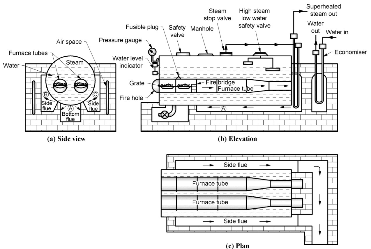
Fig. 1.4 Lancashire boiler
