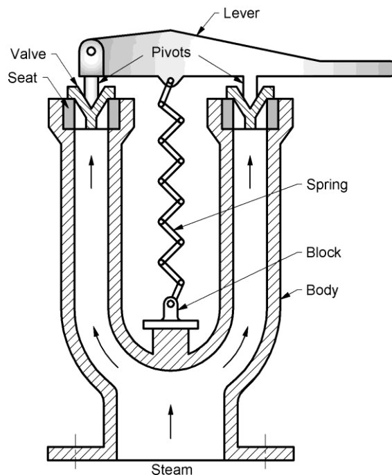
Fig. 2.9 Spring loaded valve
