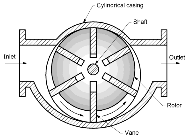
Fig. 10.5 Vane pump
