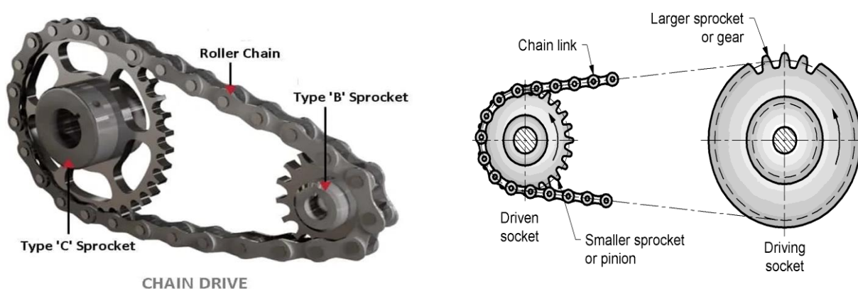
Fig. 8.18 Chain Drive
