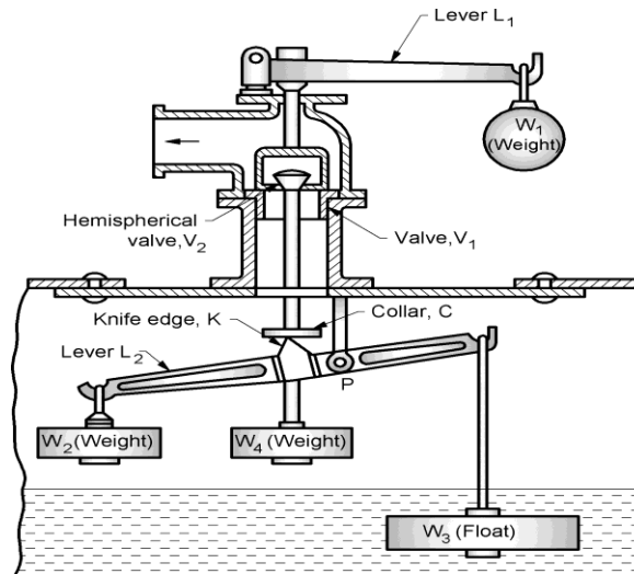
Fig. 2.10 High steam and low water safety valve
