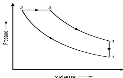
Fig 3.5 p-v diagram of two stroke diesel engine
