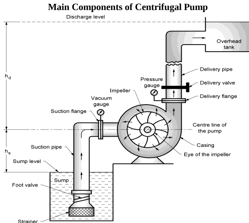
Fig. 10.3 Components of Centrifugal Pump
