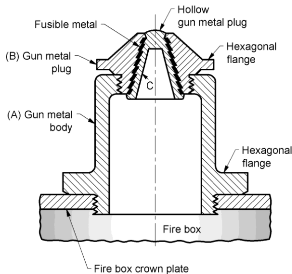
Fig. 2.6 Fusible plug
