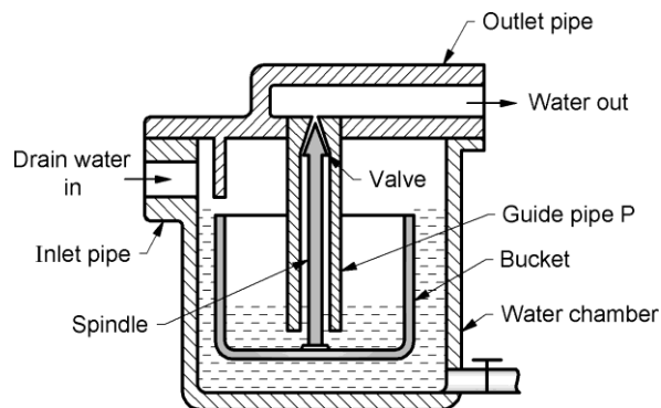
Fig. 2.17 Steam trap
