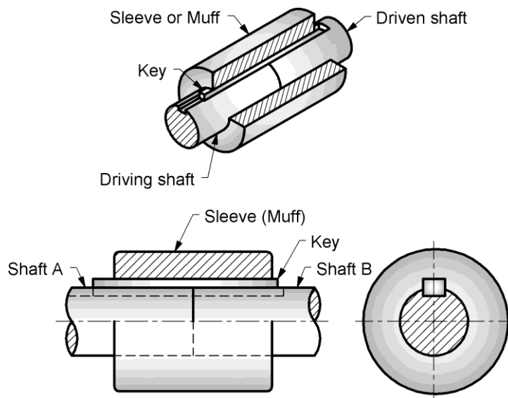
Fig. 7.2: Sleeve or box or muff coupling
