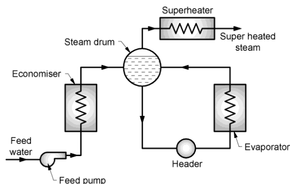
Fig. 1.1: Natural circulation boiler
