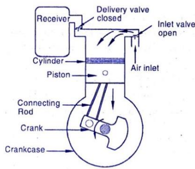
Fig. 5.2.Suction Stroke
