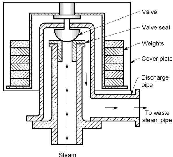
Fig. 2.7 Dead weight safety valve
