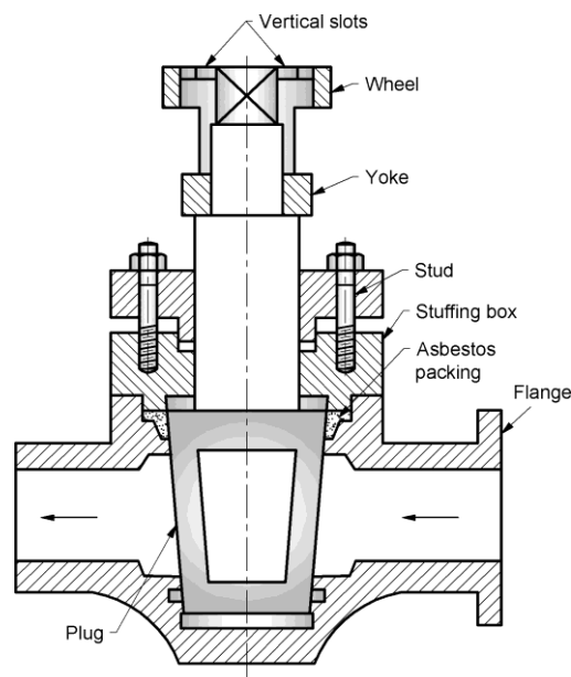
Fig. 2.5 Blow off cock
