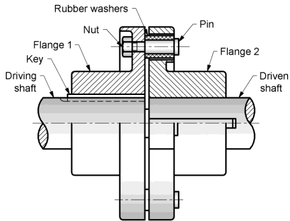
Fig. 7.5: Bush-pin type flange coupling
