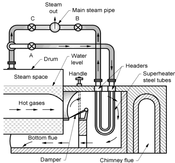
Fig. 2.14 Superheater
