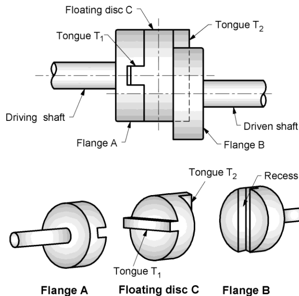
Fig. 7.6: Oldham's coupling
