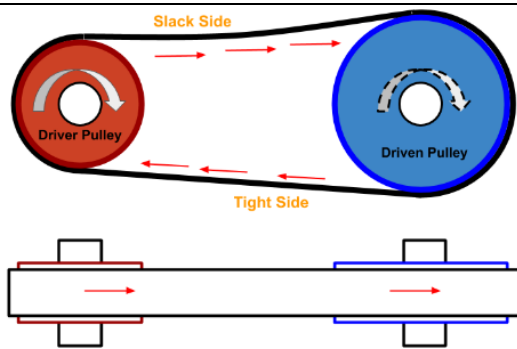
Fig 8.7 Open belt drive
