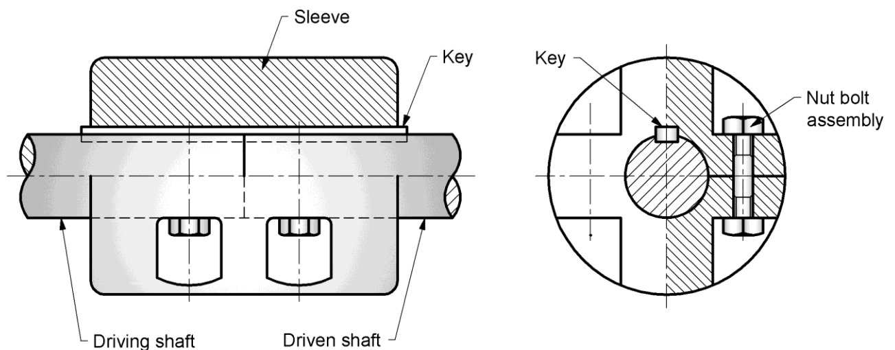
Fig. 7.3 : Split muff or clamp or compression coupling
