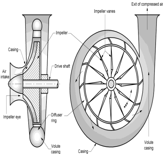
Fig. 5.10 Centrifugal Air Compressor
