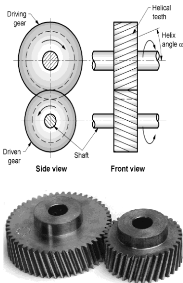
Fig8.21 Helical Gear
