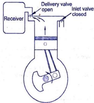
Fig. 5.3 Compression &amp; Delivery Stroke
