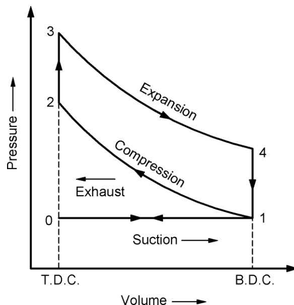
Fig. 3. 3: p-v diagram of four stroke petrol engine
