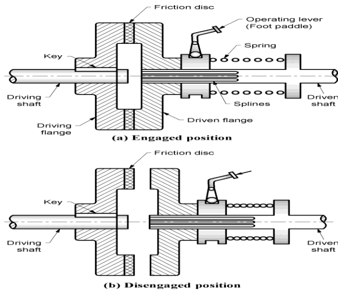
Fig. 7.8 Single disc or single plate clutch
