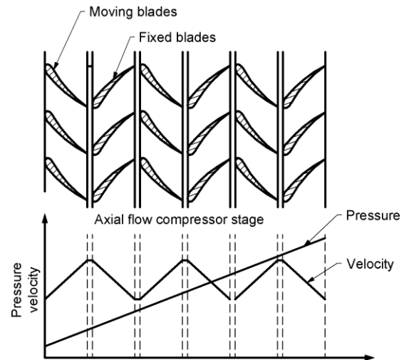
Fig. 5.13 Pressure and velocity variation in Axial Flow Compressor
