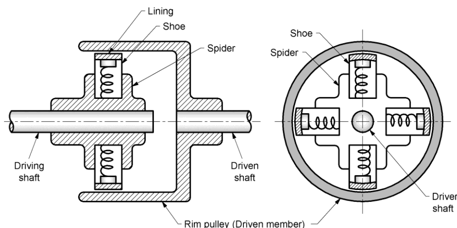
Fig. 7.10 Centrifugal clutch
