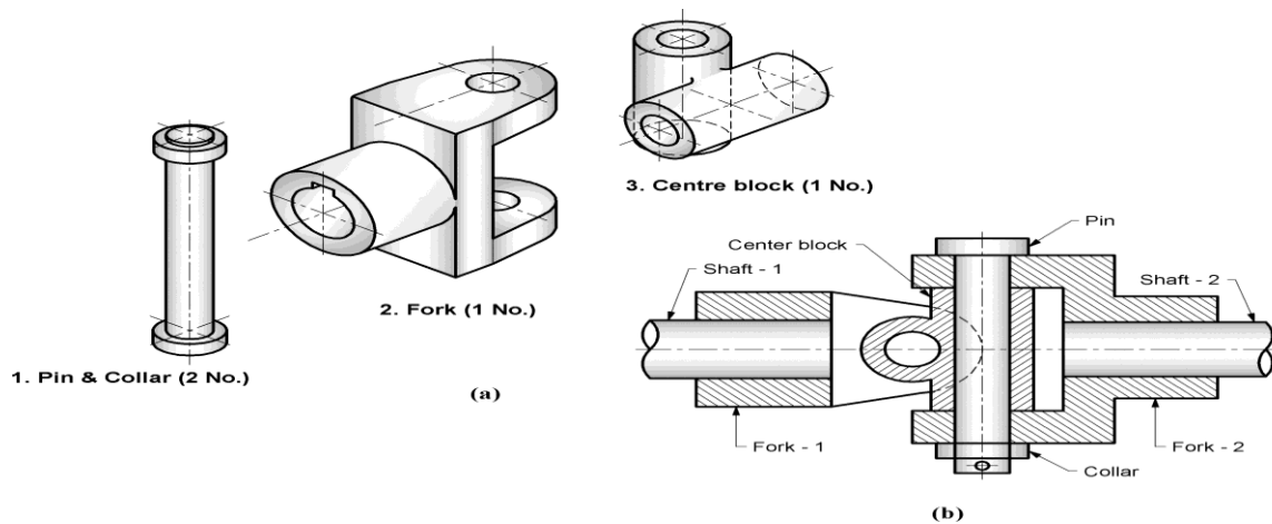
Fig. 7.7 Universal coupling or Hooke's joint
