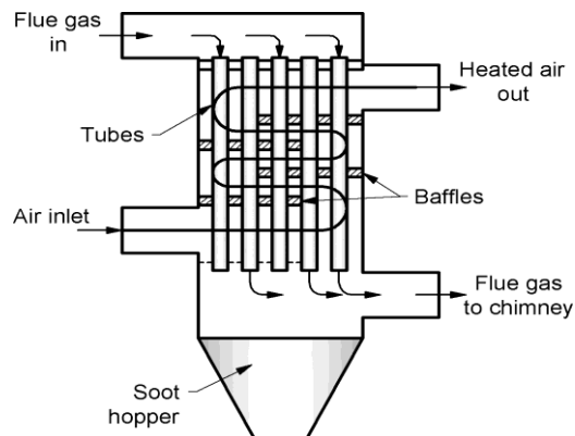
Fig. 2.15 Air pre-heater
