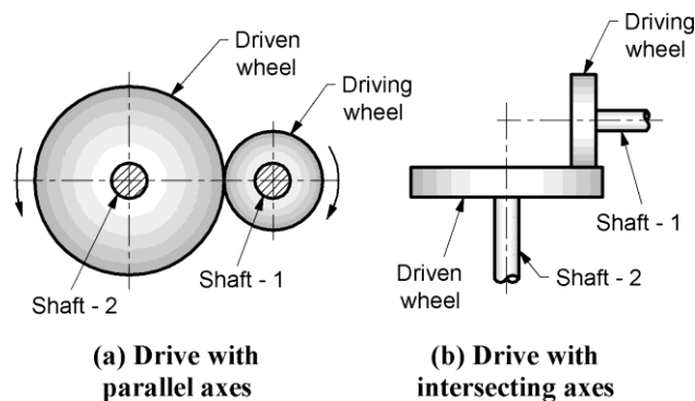
Fig 8.19 Gear Drive And Friction Drive
