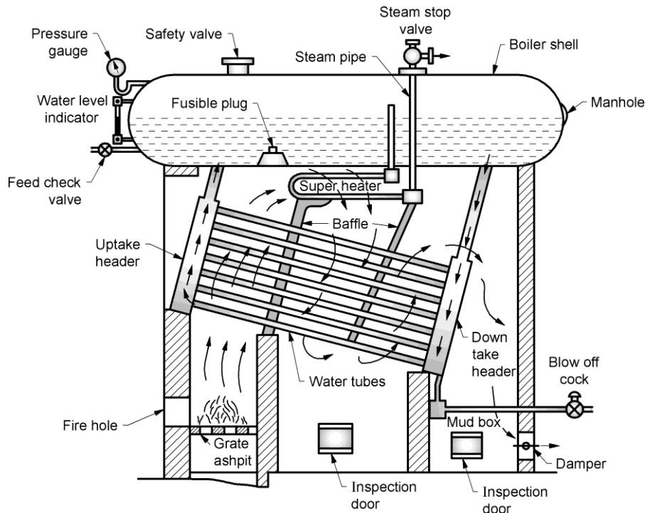
Fig. 1.5 Babcock and Wilcox boiler
