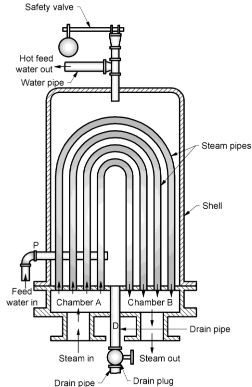
Fig. 2.13 Exhaust steam feed water heater
