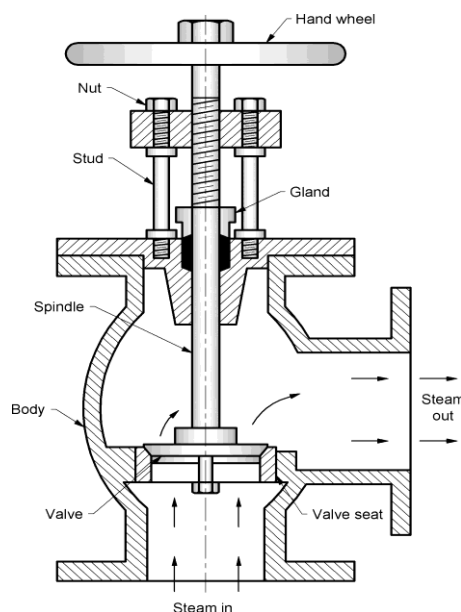
Fig. 2.3 Steam stop valve
