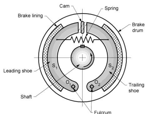
Fig. 7.14 Internal expanding shoe brake
