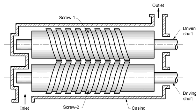
Fig. 10.6 Screw pump
