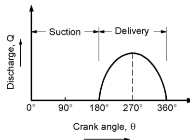
Fig.10.2 Discharge ( Q ) v/s Crank angle ( \theta ) variations for single acting pump
