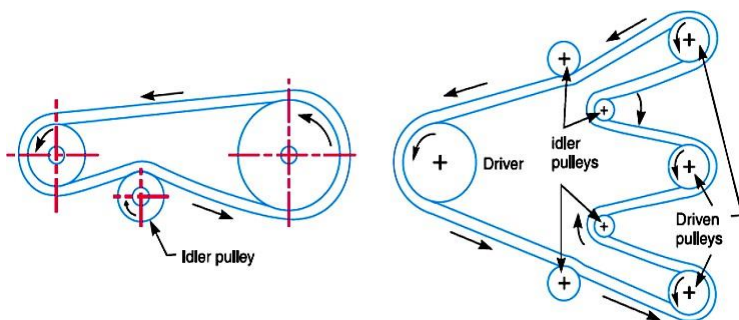
Fig 8.10 Belt drive with Idler pulley
