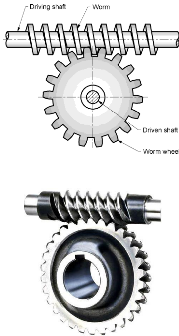
Fig 26 Worm and Worm wheel
