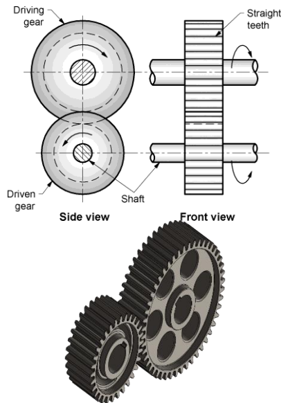
Fig 8.20 Spur Gear
