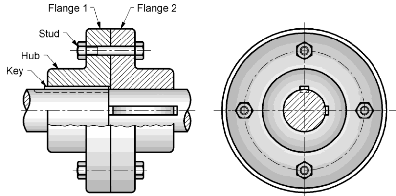
Fig. 7.4(a) :Unprotected type flange coupling
