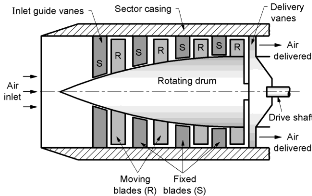
Fig 5.12 Axial Flow Air Compressor
