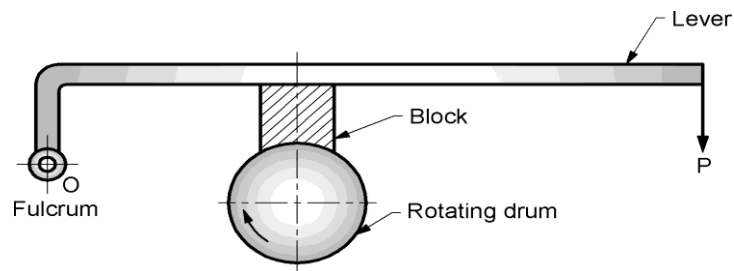
Fig. 7.11 Single block or shoe brake
