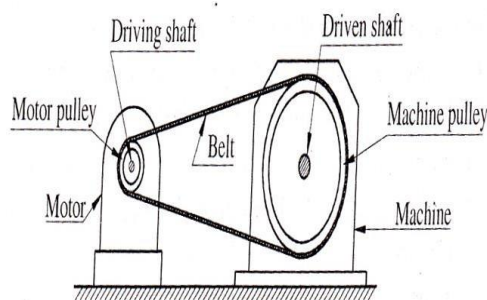
Fig.8. 1 Individual drive
