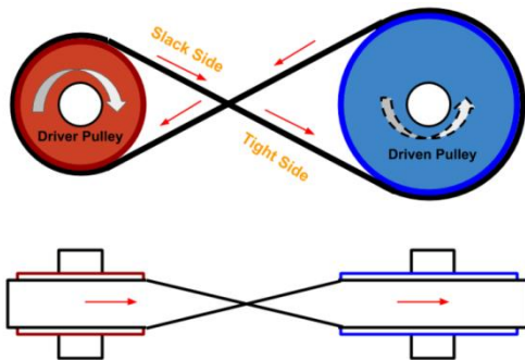
Fig 8.8. Cross Belt Drive
