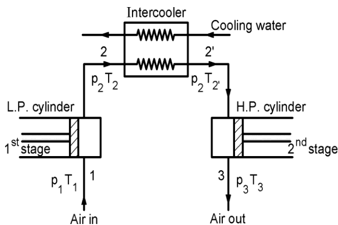
Fig.5.6 , Two Stage Compression
