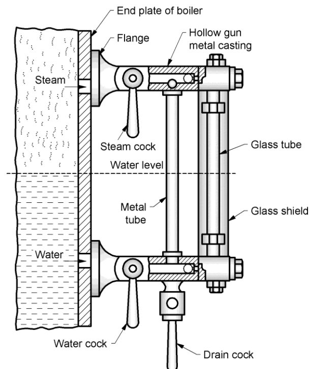
Fig. 2.2 Water level indicator
