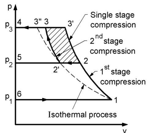
Fig.5.7 , P-V Diagram for two stage compression for comparison
