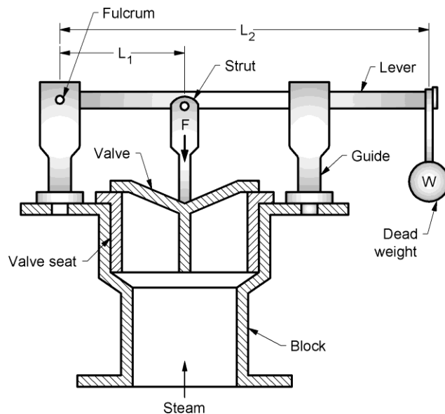
Fig. 2.8 Lever loaded valve
