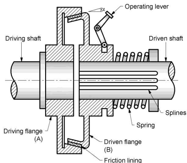
Fig. 7.9 Cone clutch
