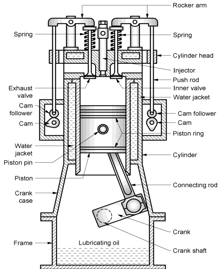
Fig.3.1): I.C. engine parts
