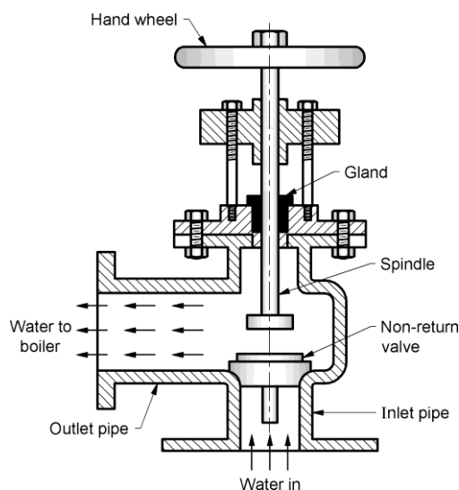
Fig. 2.4 Feed check valve
