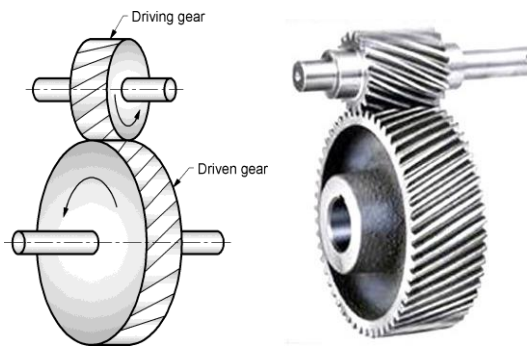
Fig 8.23 Spiral Gear
