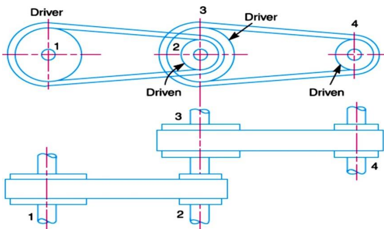
Fig.8.13 Compound beltdrive
