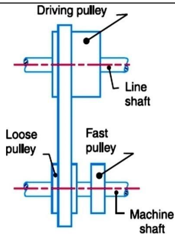
Fig 8.11 Fast and loose pulley
