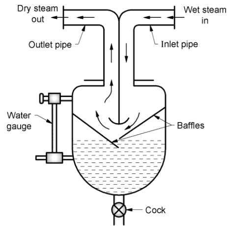
Fig. 2.16 Steam separator
