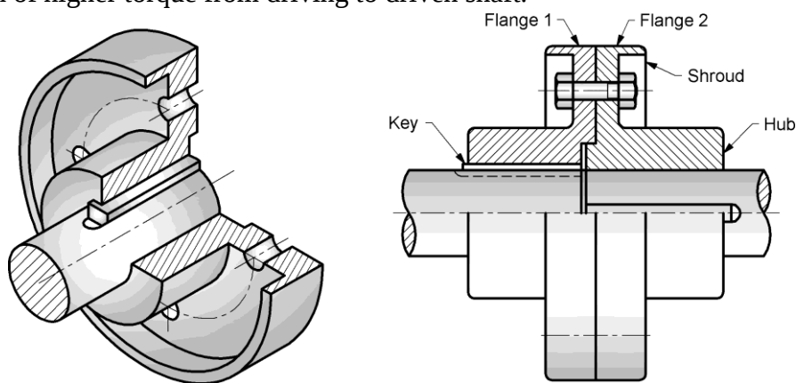
Fig. 7.4(b) Protected type flange coupling
