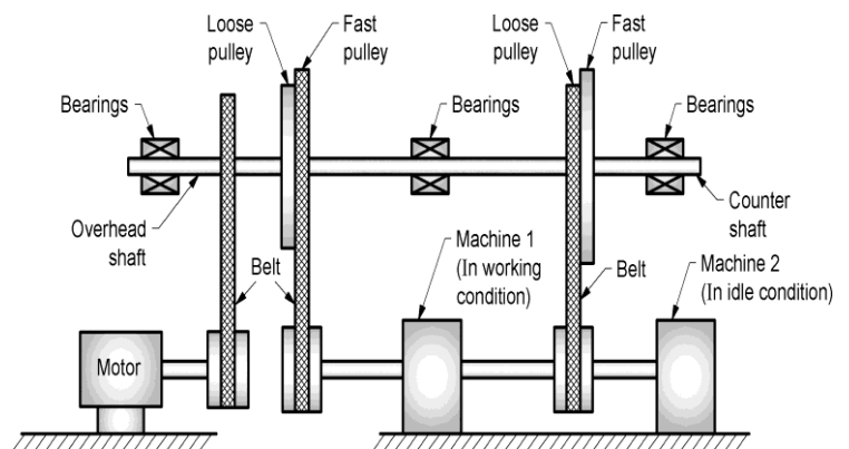
Fig. 8.2 Group Drive
