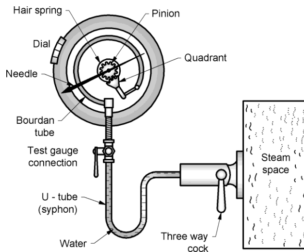
Fig. 2.1 Pressure gauge
