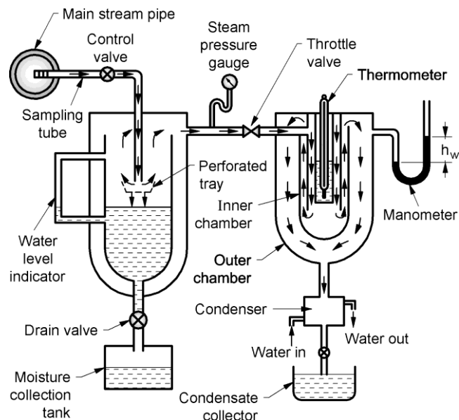
Fig. 9.1 Combined separating and throttling calorimeter
