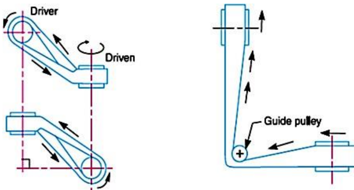
Fig 8.9 Quarter turn belt drive
