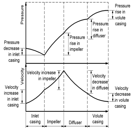
Fig.5.11 Pressure and velocity variation in a centrifugal compressor
